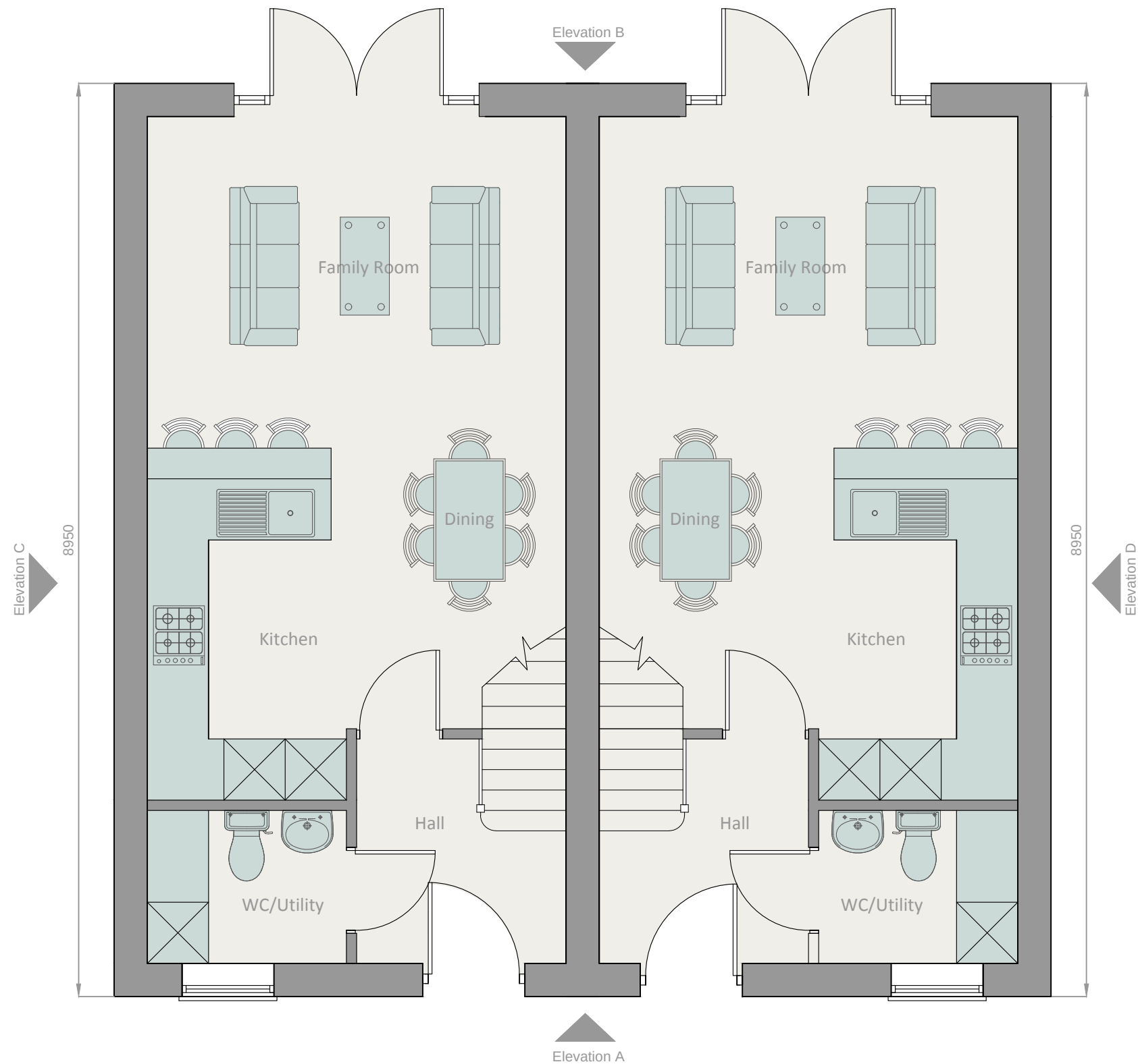
1 Ground Floor Plans 1:50
