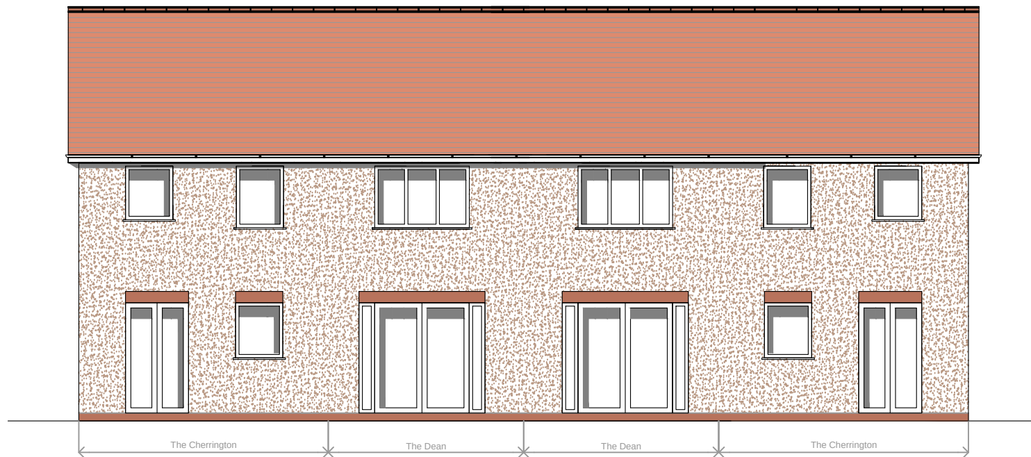
Rear Elevation B
