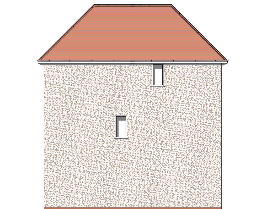
4 Side Elevation D 1:100
