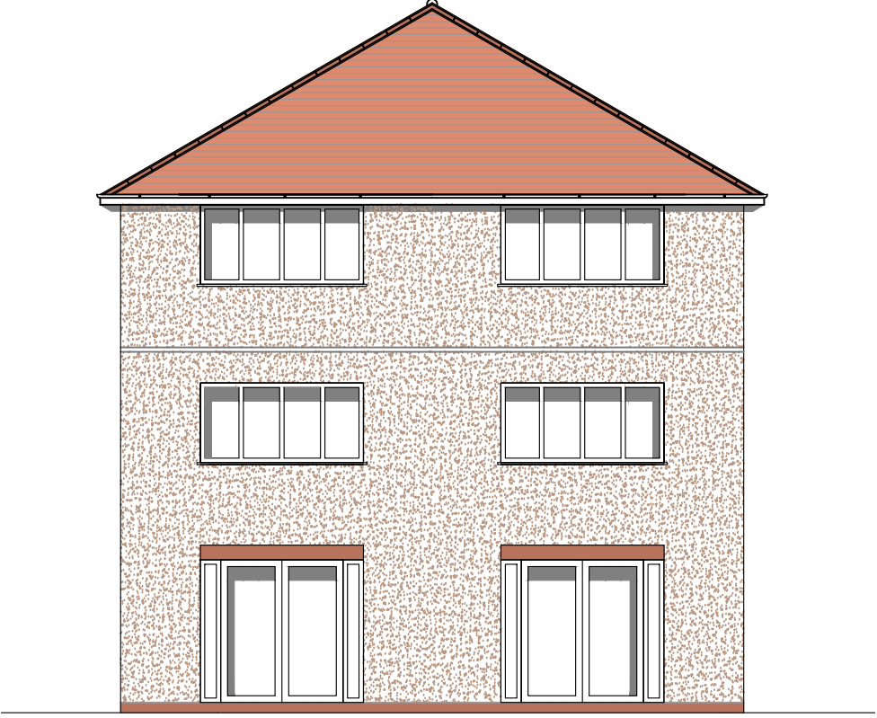
2 Rear Elevation B 1:100
